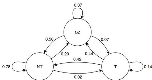
Figura 7 – VTMG (Detoxify) Roblox
