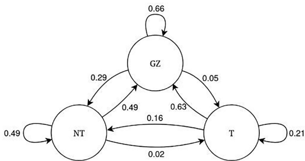
Figura 11 – VTMG (Perspective API) Julia MineGirl
